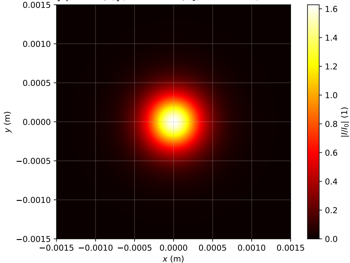
Intensity profile I(x, y, z = 2.388m)/I_0 , P_{in}=0.9P_{cr} , artificial time
